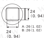
A1137B PLCC 25x25 (0.98x0.98)
