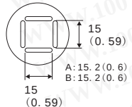
A1126B QFP 14x14 (0. 55x0. 55)
