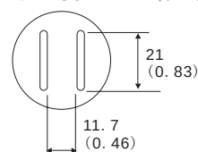
A1257B SOP 11x21 (0.43x0.83)
