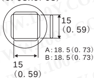
A1135B PLCC 17.5x17.5 (0.68x0.68)
