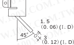
A1142B Bent single 1.5x3 (0.06x0.12)
