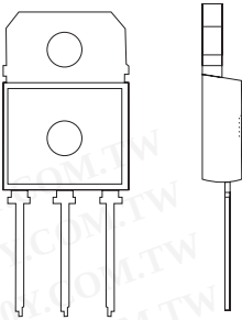
TO-218AB
