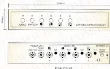
Rear Panel
