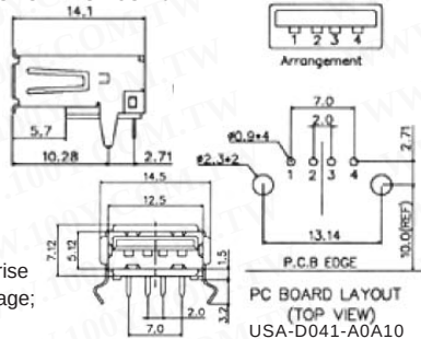
USB SERIES A USA-04
