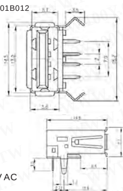
USB SERIES A USA-04
