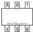
MIC94060/1 SC-70-6 (C6)
