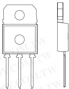
TO-218AB
