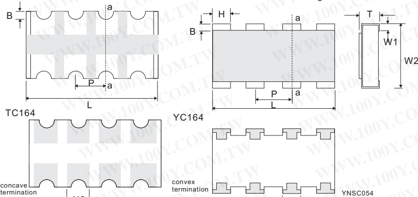
Fig. 3 YC/TC164 series chip resistors dimension
