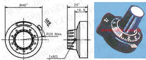
24 Multi-Turn Dial Mechanisms
