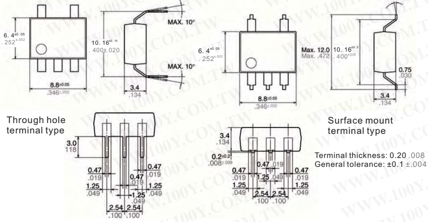
DIP6 Wide Terminal Type APT1212W(A), APT1222W(A), APT1232W(A)
