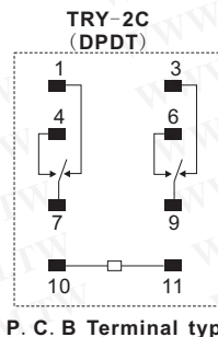
P. C. B Terminal type
