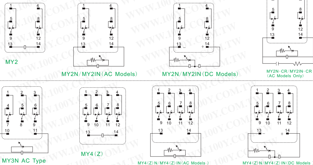
Terminal arrangement/internal connections (bottom view)
