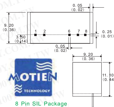
8 Pin SIL Package
