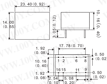
16 PIN DIL Package
