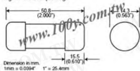
Fig. 1: 1-50 Amp Range
