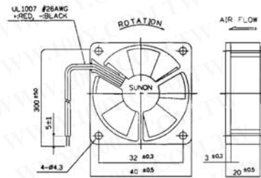
UNIT: mm KD1204PKB2(2)
