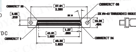
CA-68MDS-A-0
